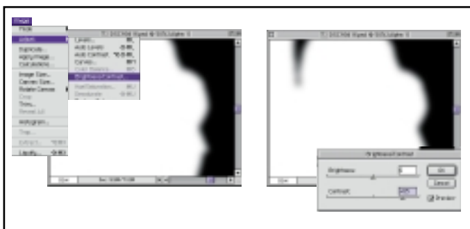
Image\Adjust\Brightness/Contrast
