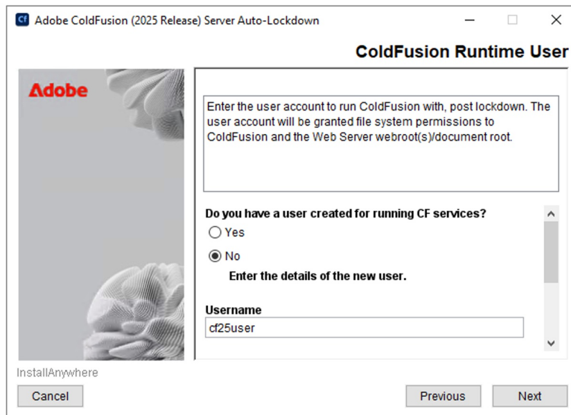
Lockdown Installer: ColdFusion Runtime User
