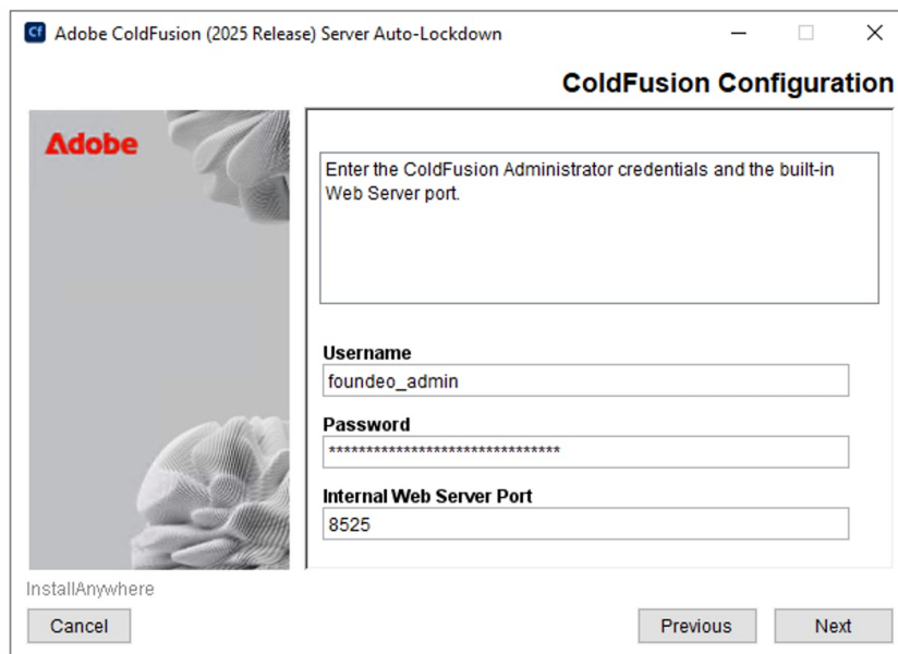
Lockdown Installer: ColdFusion Administrator Configuration
